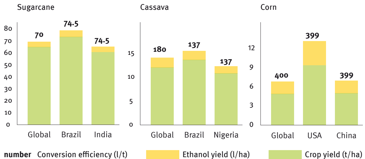
Figure 26: Biofuel yields (FAO, 2008)
