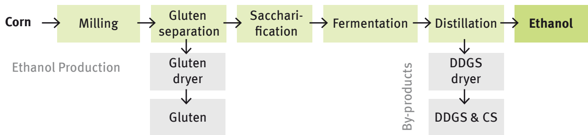
Figure 25: Simplified corn ethanol production process
