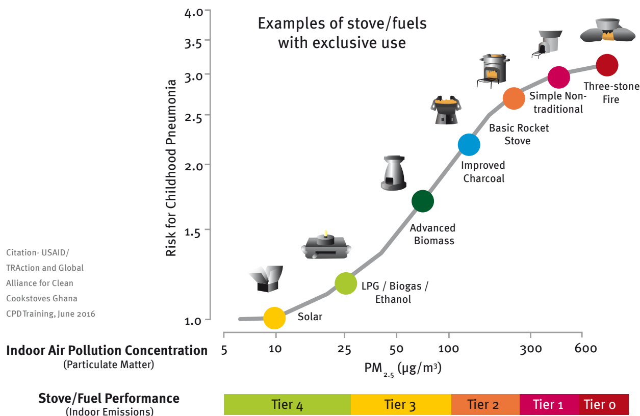
Figure 10: Emissions of PM 2.5 from cooking stoves related to risk of childhood pneumonia (USAID/TRAction and Global Alliance for Clean Cookstoves, 2016)
