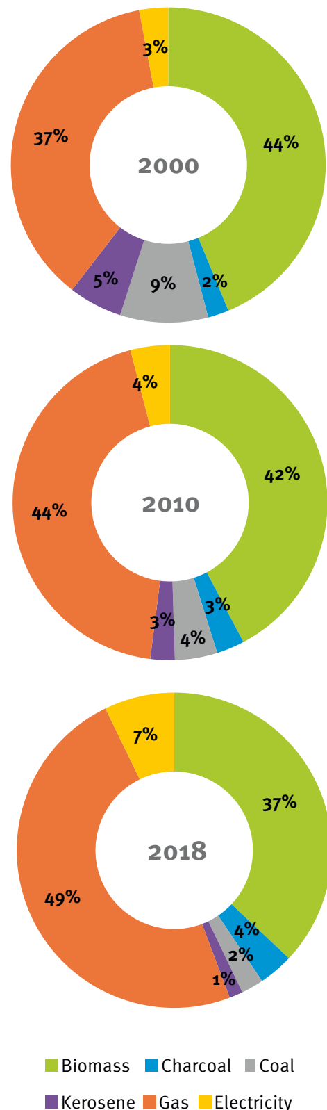
Figure 17: Comparison of the percentage of people using each fuel type among low and middle-income countries in 2000, 2010, and 2018 (IEA, IRENA, UNSD, World Bank, WHO, 2020)
