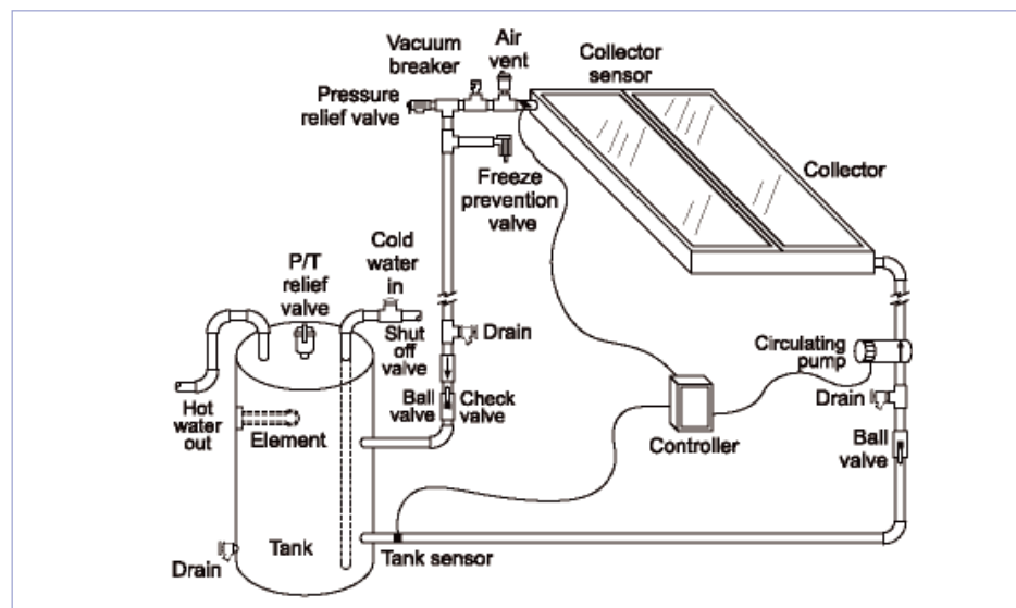
Figure 1. A solar water heating system
