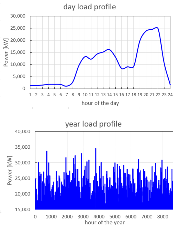
Figure 4. Typical load curves for a smaller grid in Zambia, one typical day and one year profiles
