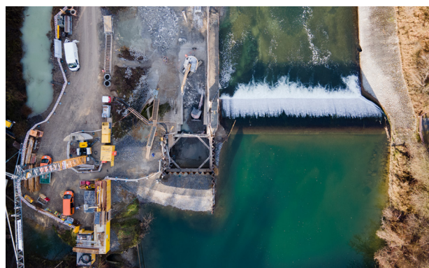
Figure 5. Excavation and Partial Removal of the Weir Structure for the New HSPP
